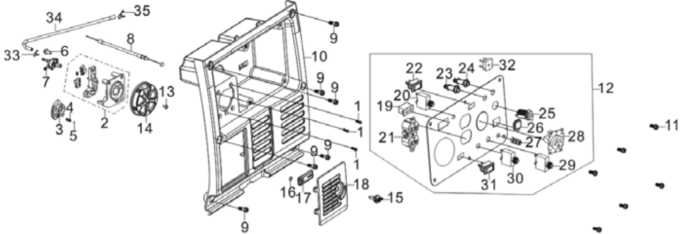
Fig. 14 - Control Panel Assembly
