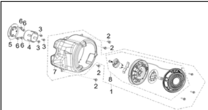
Fig. 7 - Recoil Starter
